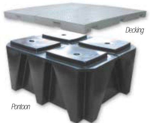
Pontoon Decking & Pontoon Float FL3050 - FL3023
